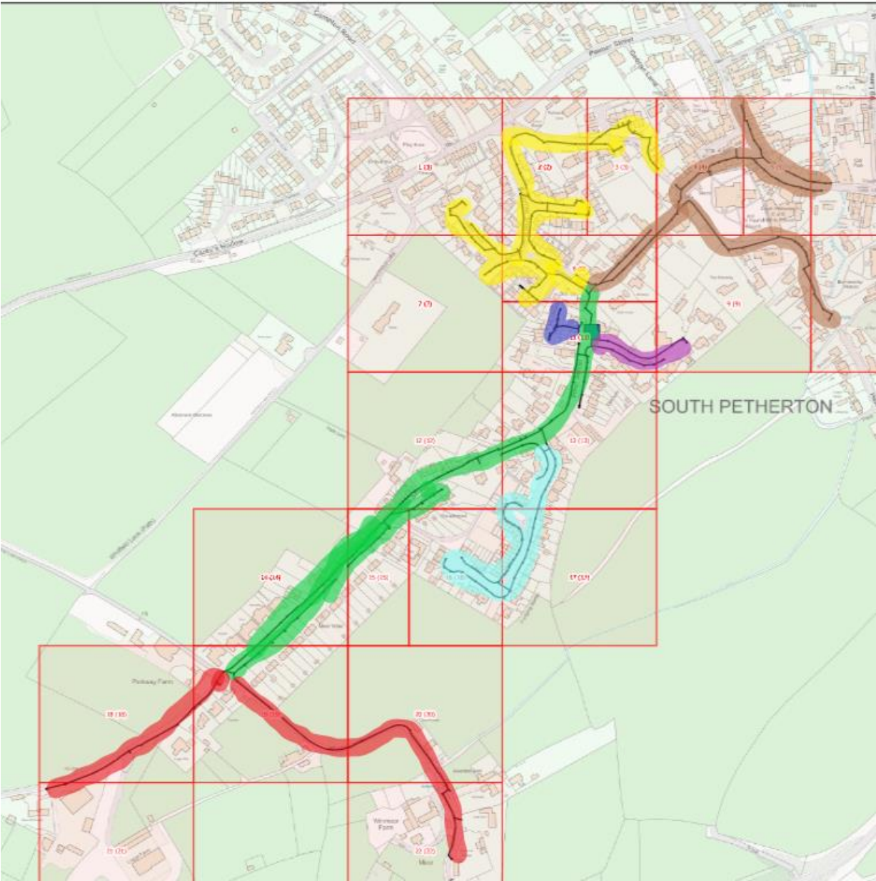
Civils drawing South Petherton (South West) 02 – SW-SPEN-02
